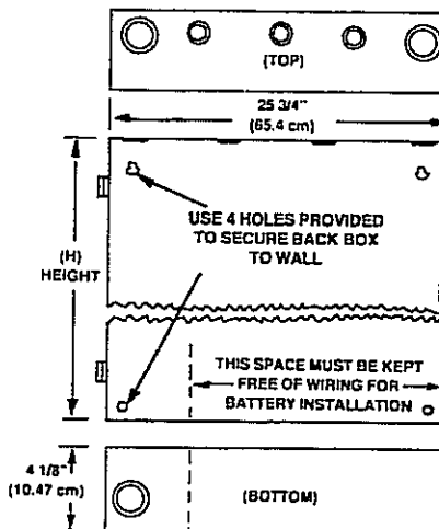
Figure 6 – Back Box Mounting Instructions
