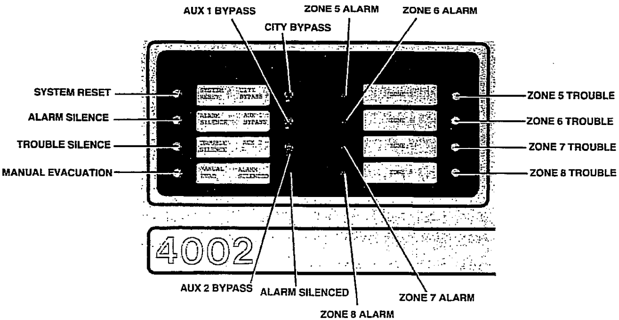
Figure 2 – 4002 Operator Switches And Indicators
