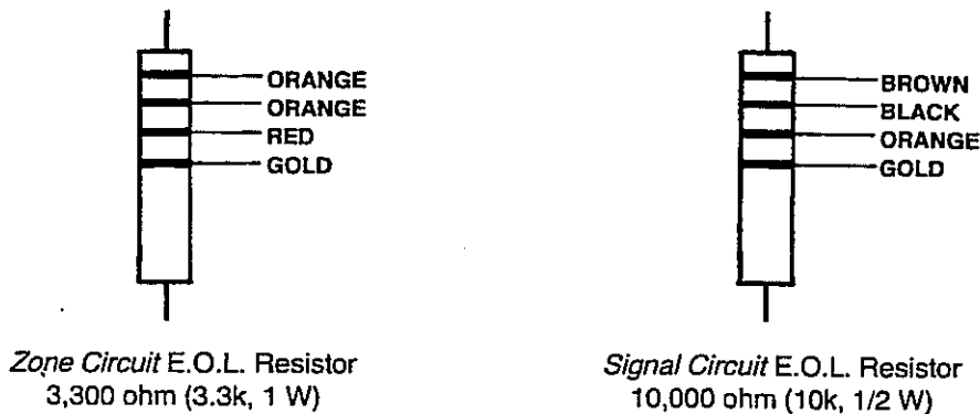
Figure 5 – E.O.L. Resistors
